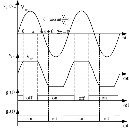
Figure 5: Voltages and control signal in dual side switching.
