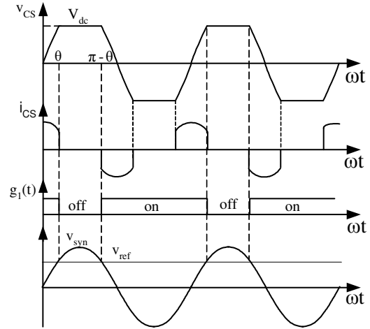
Figure 7: Voltage and current waveforms of C_s .
