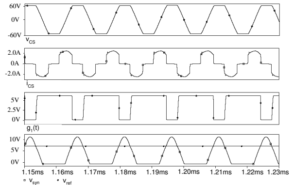
Figure 8: Simulation results of dual side switching.
