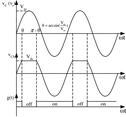
Figure 4: Voltages and control signal in single side switching.
