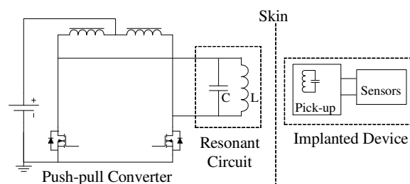
Figure 1: Basic configuration of a WP supply system.
