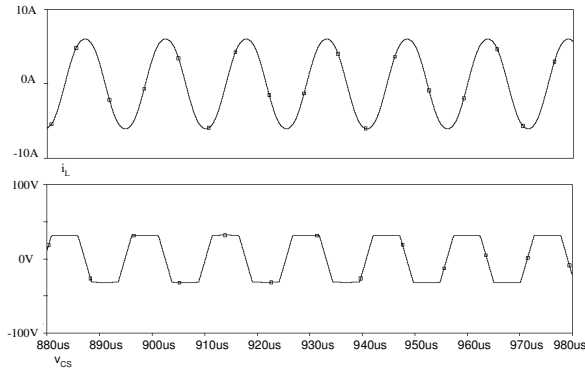
(b) L=30\mu\text{H}
