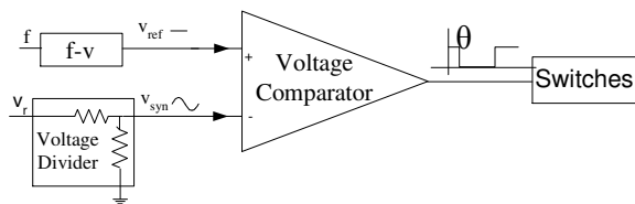
Figure 6: Basic structure of phase shift control.
