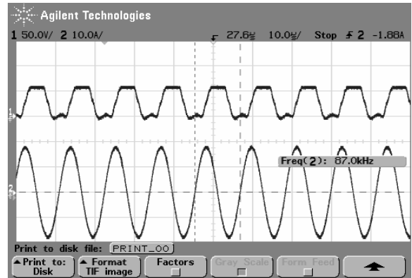
Figure 10: Experimental results of switched capacitor voltage and inductor current.
