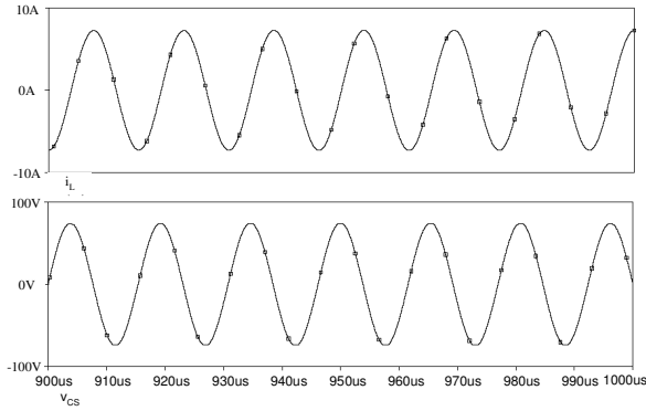
(a) L=25\mu\text{H}
