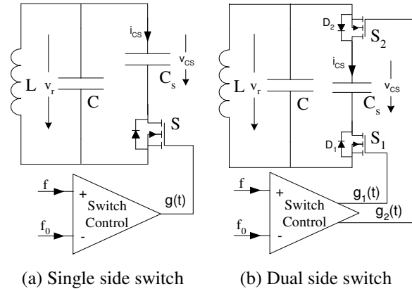
Figure 3: Switched capacitors in a resonant tank.
